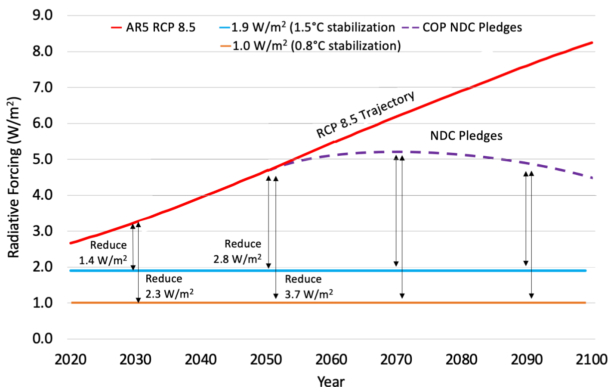
Figure B. 1 Illustrative example showing the RF reduction required to maintain the global mean temperature at +1.5^{\circ}\text{C} (i.e., 1.9 \text{ W/m}^2 ) or below +0.8^{\circ}\text{C} (i.e., 1.0 \text{ W/m}^2 ) when compared to RCP 8.5. This figure assumes that substantial effects of 2 nd round of NDCs pledged in 2021 begin to be seen at 2050. While there is uncertainty regarding future RF levels included in this figure, the most widely accepted estimates by the IPCC in its Representative Concentration Pathways (RCPs) scenarios project a rise to about +3.0 \text{ W/m}^2 by 2030—a rate that, if sustained, would eventually lead to an increase in average global temperature to over +2.0^{\circ}\text{C} . As described in the IPCC SR1.5, maintaining RF at +1.9 \text{ W/m}^2 will provide a 50% likelihood of stabilization of the GST anomaly at about +1.5^{\circ}\text{C} . (Source: IPCC, 2018)
