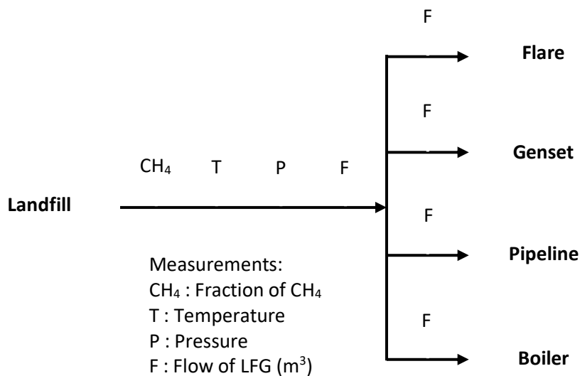
Figure 1: Suggested Arrangement of LFG Metering Equipment (recreated based on CAR U.S. Landfill Protocol)
